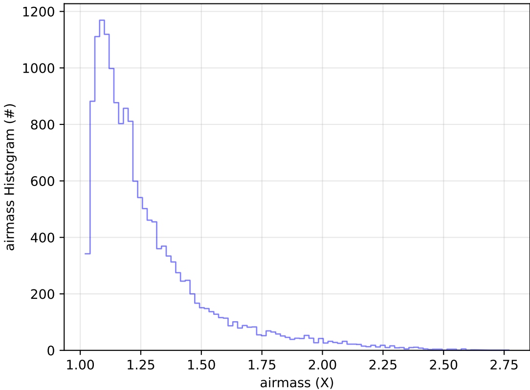
ddf_acor_sf25_lsf40_lsr20_v3.4_10yrs Yr 1 u band: airmass Histogram
