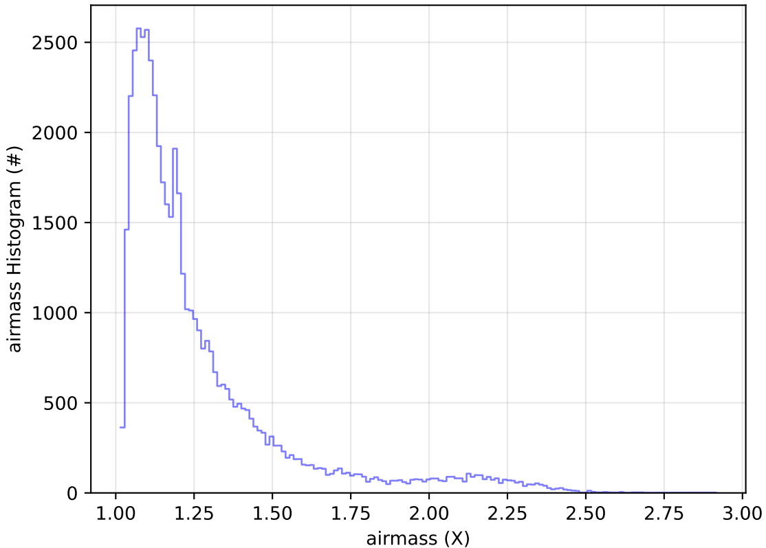
ddf_acor_sf25_Isf40_Isr20_v3.4_10yrs Yr 1 r band: airmass Histogram
