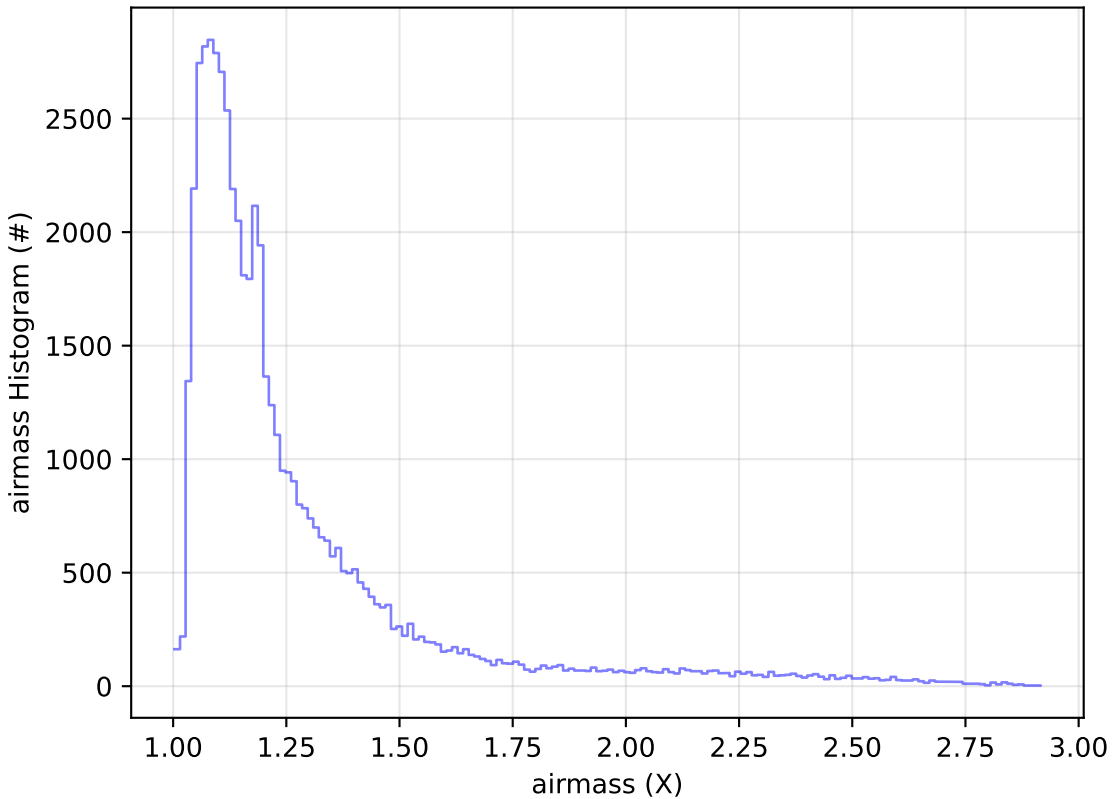
ddf_acor_sf25_lsf40_lsr20_v3.4_10yrs Yr 1 i band: airmass Histogram
