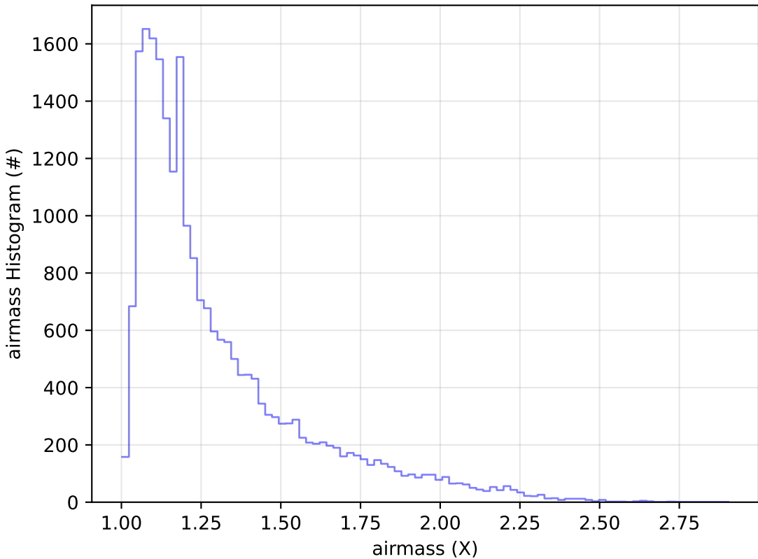
ddf_acor_sf25_lsf40_lsr20_v3.4_10yrs Yr 1 g band: airmass Histogram
