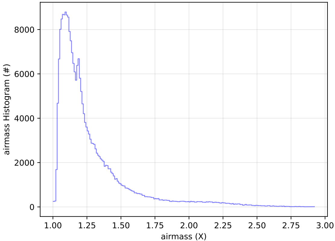
ddf_acor_sf25_lsf40_lsr20_v3.4_10yrs Yr 1 all bands: airmass Histogram
