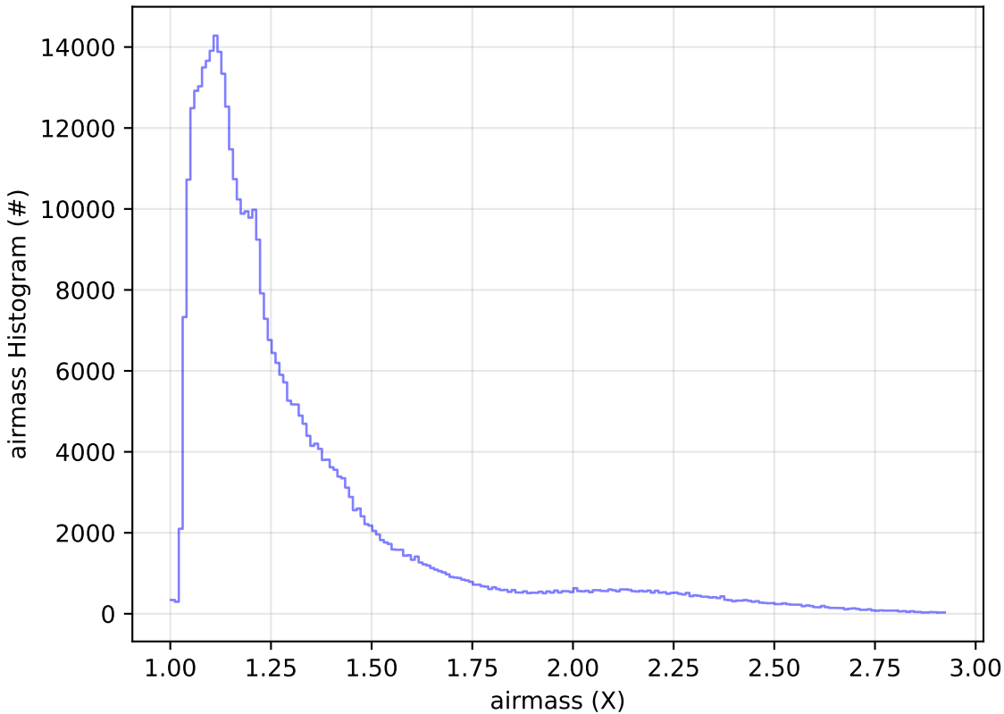
ddf_acor_sf25_lsf40_lsr20_v3.4_10yrs WFD z band: airmass Histogram
