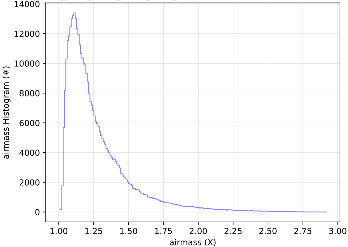
ddf_acor_sf25_lsf40_lsr20_v3.4_10yrs WFD y band: airmass Histogram
