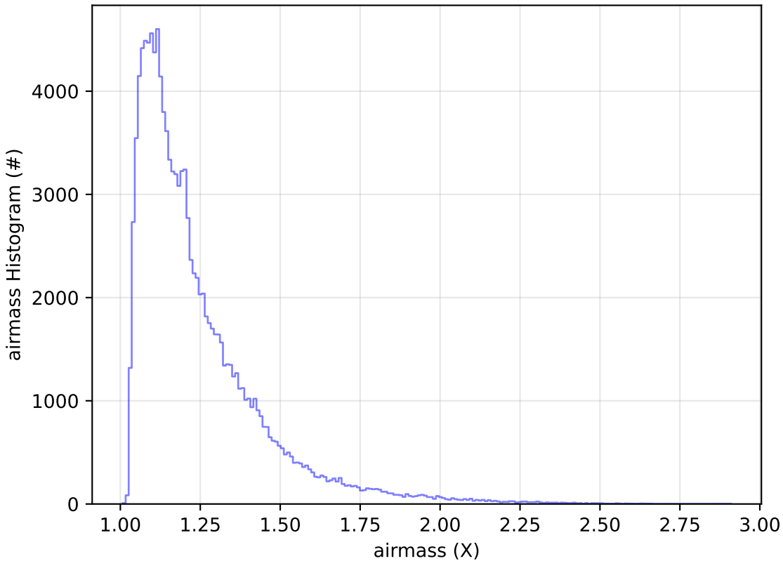
ddf_acor_sf25_lsf40_lsr20_v3.4_10yrs WFD u band: airmass Histogram
