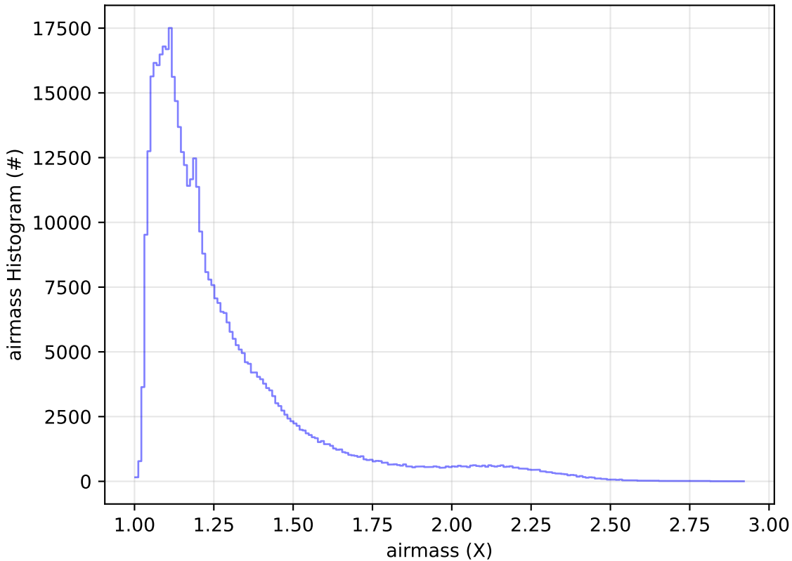
ddf_acor_sf25_Isf40_Isr20_v3.4_10yrs WFD r band: airmass Histogram
