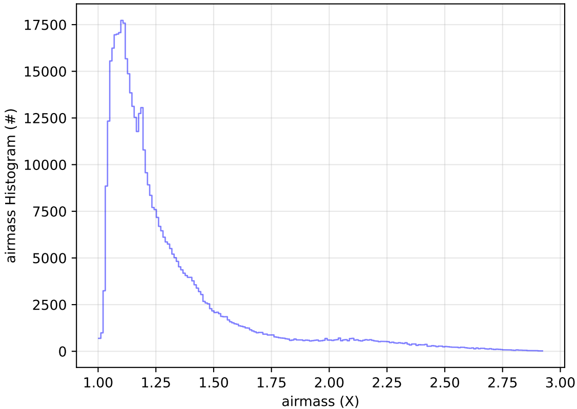
ddf_acor_sf25_lsf40_lsr20_v3.4_10yrs WFD i band: airmass Histogram
