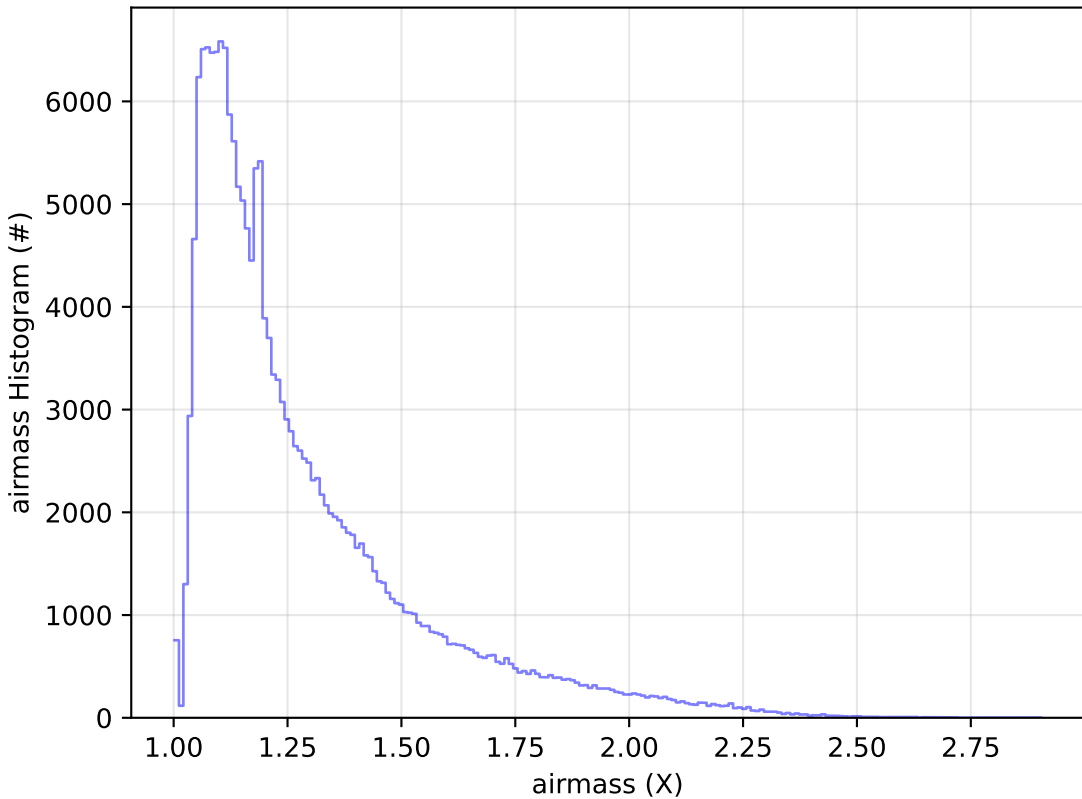
ddf_acor_sf25_lsf40_lsr20_v3.4_10yrs WFD g band: airmass Histogram
