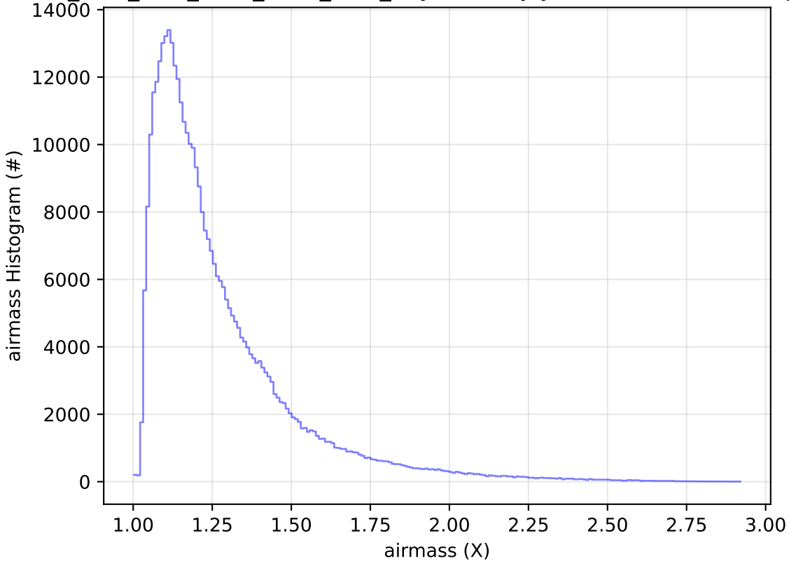
ddf_acor_sf25_lsf40_lsr20_v3.4_10yrs All sky y band: airmass Histogram
