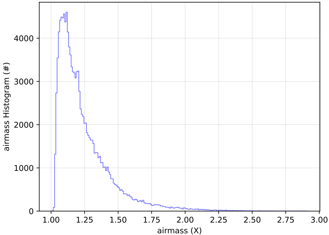
ddf_acor_sf25_lsf40_lsr20_v3.4_10yrs All sky u band: airmass Histogram
