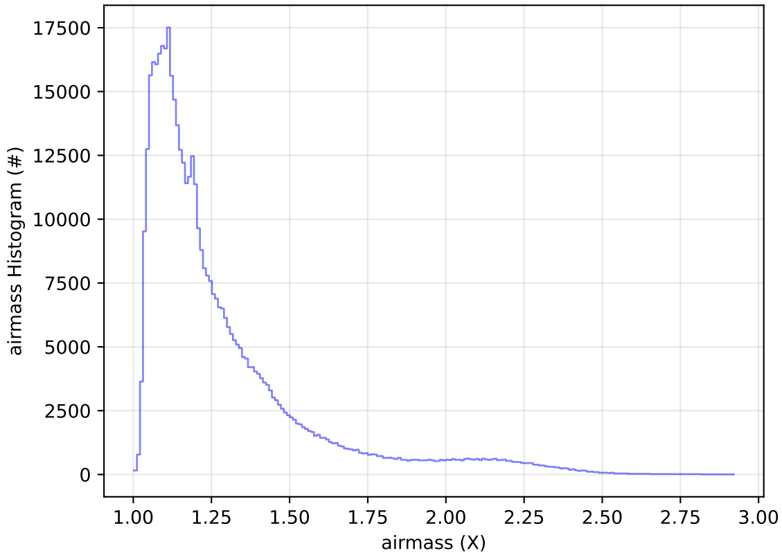
ddf_acor_sf25_lsf40_lsr20_v3.4_10yrs All sky r band: airmass Histogram
