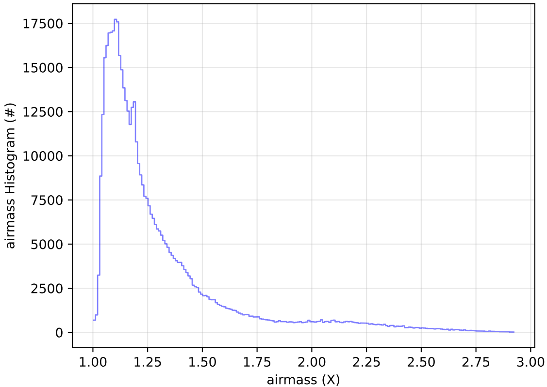
ddf_acor_sf25_lsf40_lsr20_v3.4_10yrs All sky i band: airmass Histogram
