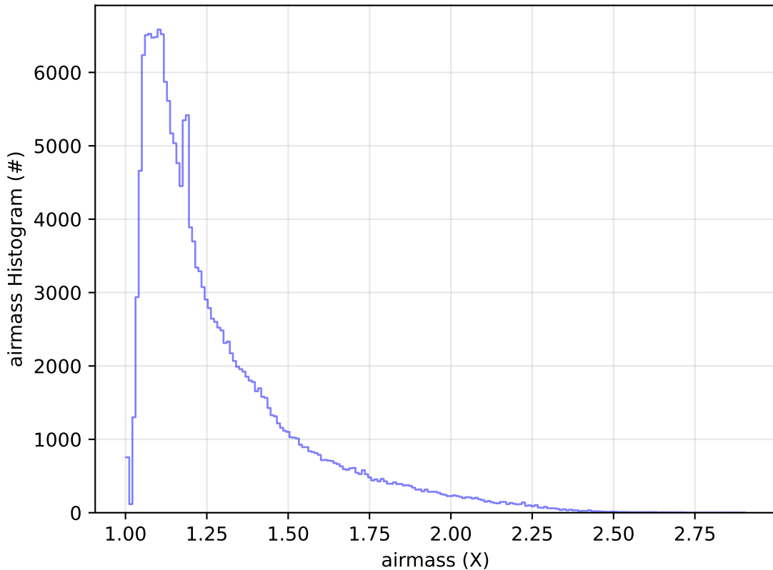
ddf_acor_sf25_lsf40_lsr20_v3.4_10yrs All sky g band: airmass Histogram
