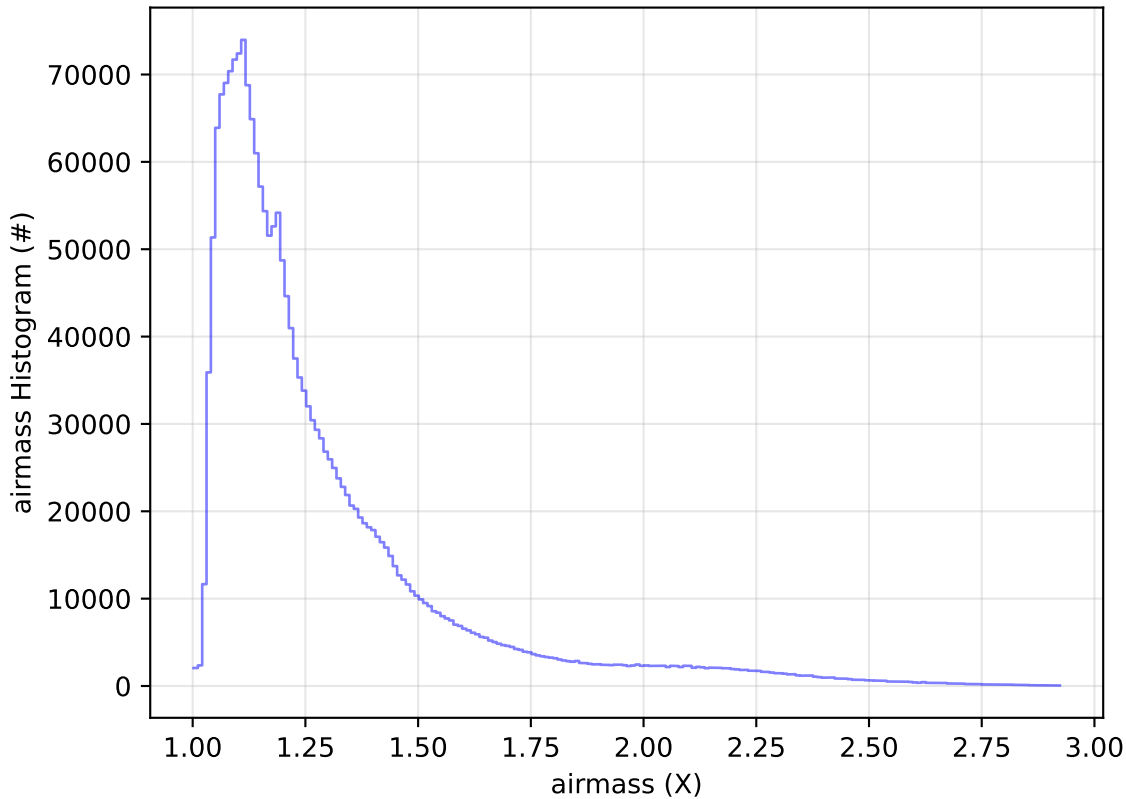
ddf_acor_sf25_lsf40_lsr20_v3.4_10yrs All sky all bands: airmass Histogram
