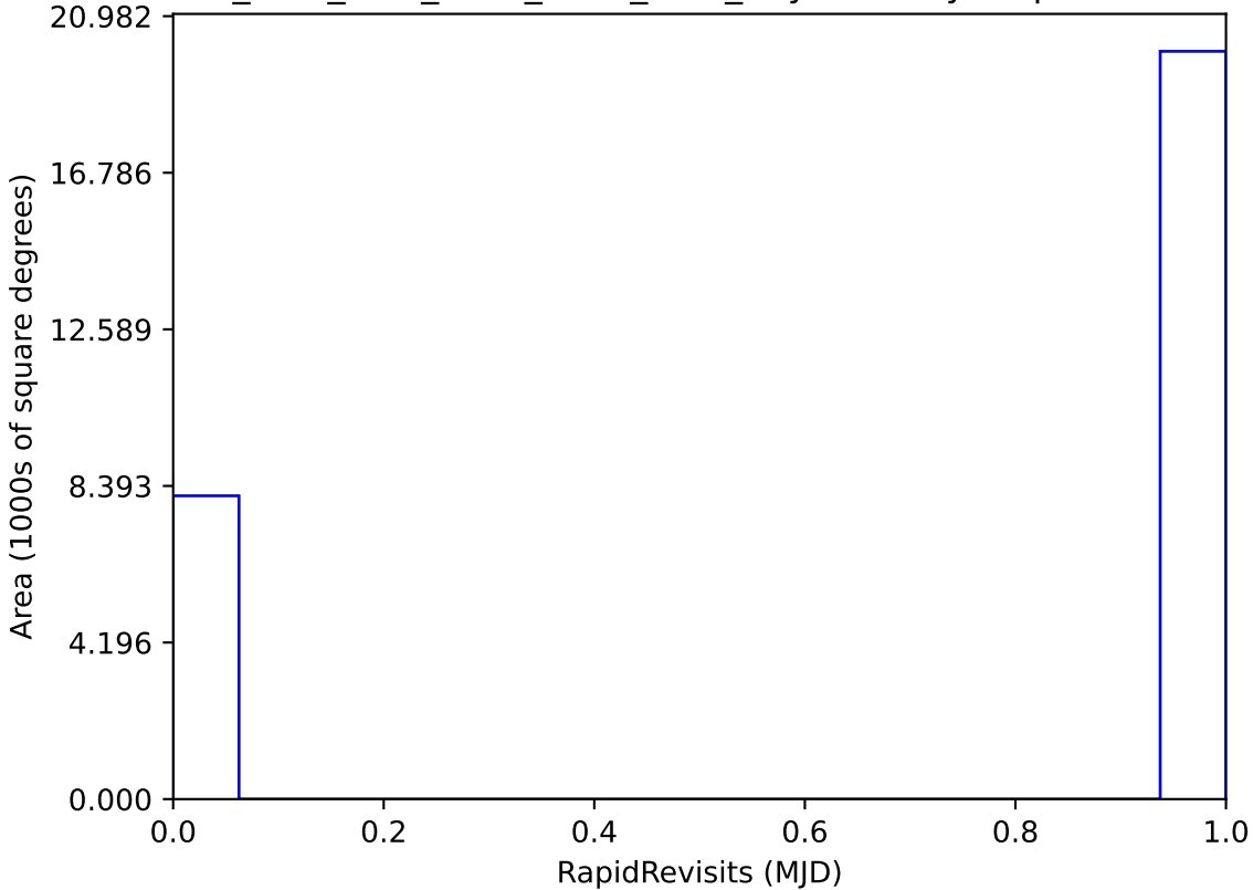
ddf_acor_sf25_lsf40_lsr20_v3.4_10yrs All sky: RapidRevisits
