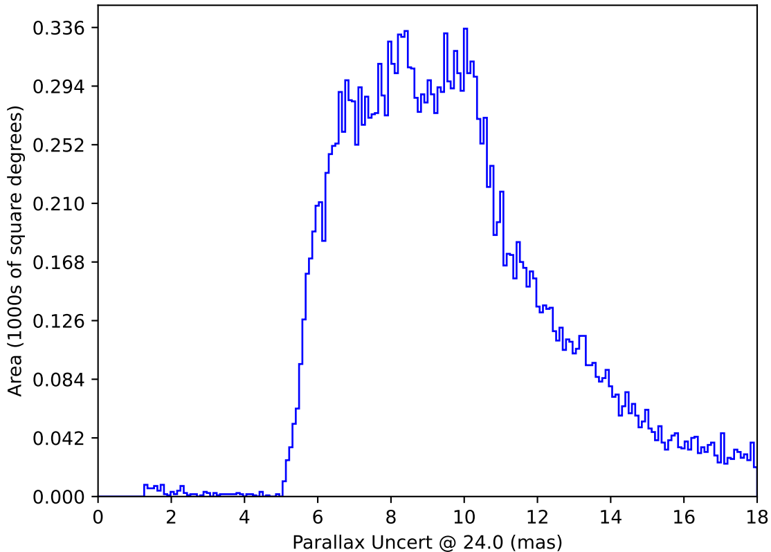
ddf_acor_sf25_lsf40_lsr20_v3.4_10yrs All sky: Parallax Uncert @ 24.0
