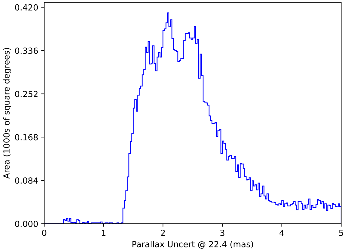
ddf_acor_sf25_lsf40_lsr20_v3.4_10yrs All sky: Parallax Uncert @ 22.4
