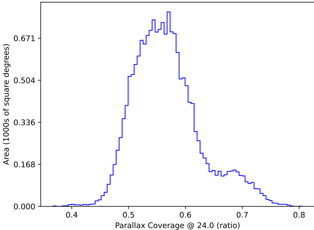
ddf_acor_sf25_lsf40_lsr20_v3.4_10yrs WFD: Parallax Coverage @ 24.0
