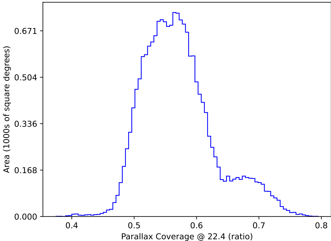
ddf_acor_sf25_lsf40_lsr20_v3.4_10yrs WFD: Parallax Coverage @ 22.4
