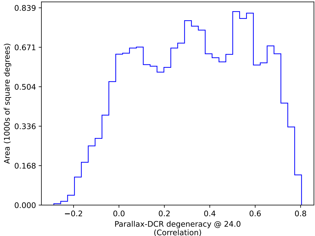
ddf_acor_sf25_lsf40_lsr20_v3.4_10yrs WFD: Parallax-DCR degeneracy @ 24.0
