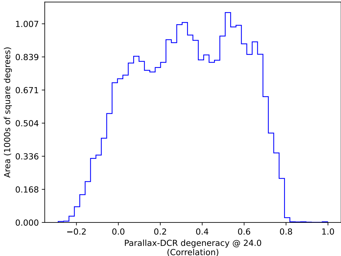
ddf_acor_sf25_lsf40_lsr20_v3.4_10yrs All sky: Parallax-DCR degeneracy @ 24.0
