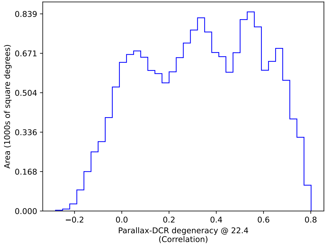
ddf_acor_sf25_lsf40_lsr20_v3.4_10yrs WFD: Parallax-DCR degeneracy @ 22.4
