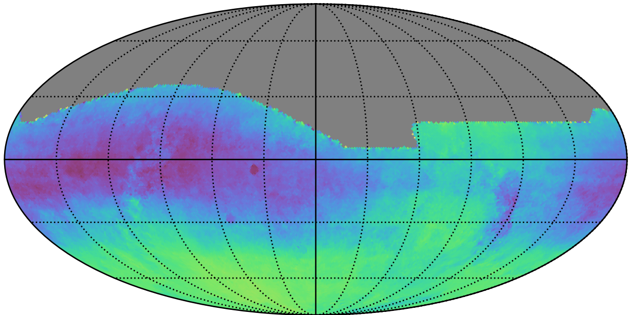
ddf_acor_sf25_lsf40_lsr20_v3.4_10yrs All sky: Parallax-DCR degeneracy @ 22.4
