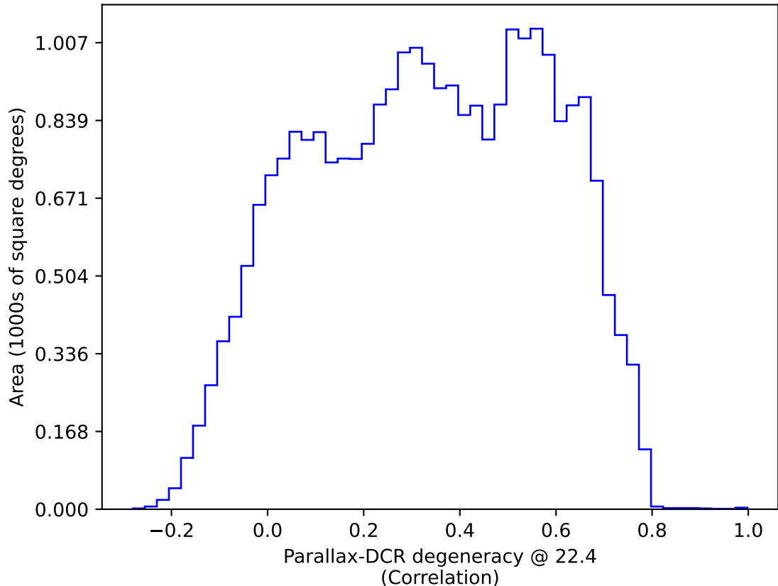
ddf_acor_sf25_lsf40_lsr20_v3.4_10yrs All sky: Parallax-DCR degeneracy @ 22.4
