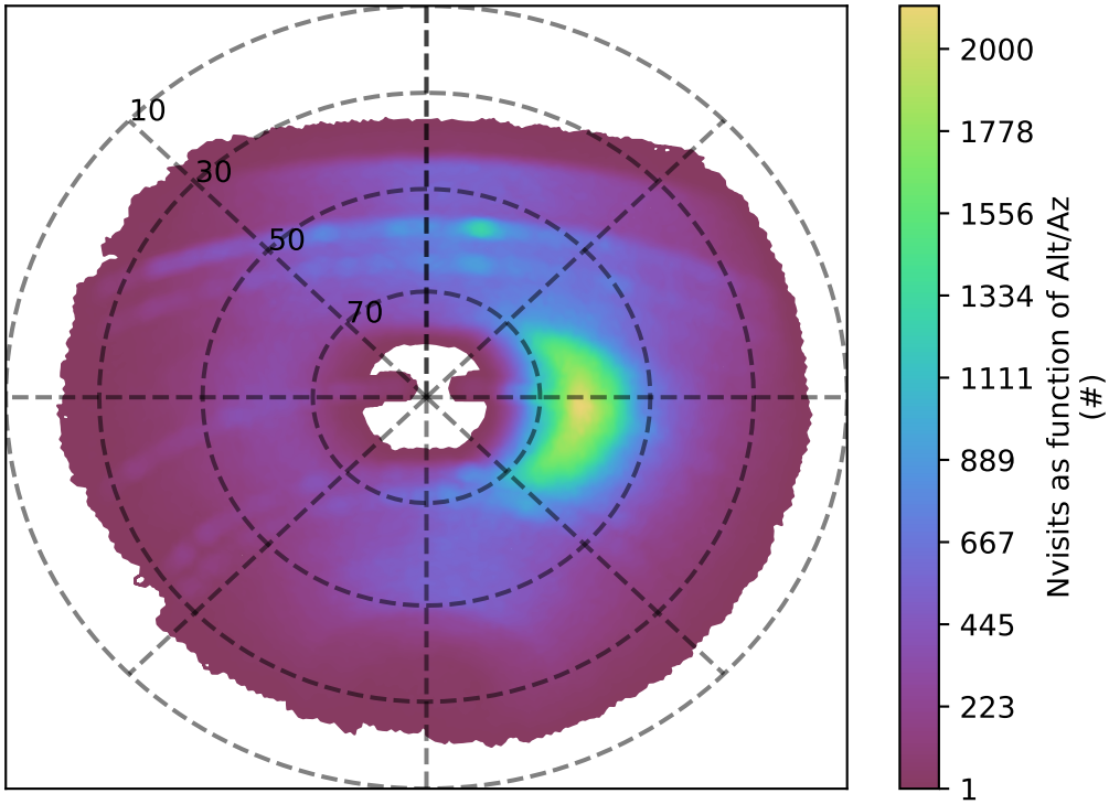
ddf_acor_sf25_lsf40_lsr20_v3.4_10yrs y band: Nvisits as function of Alt/Az
