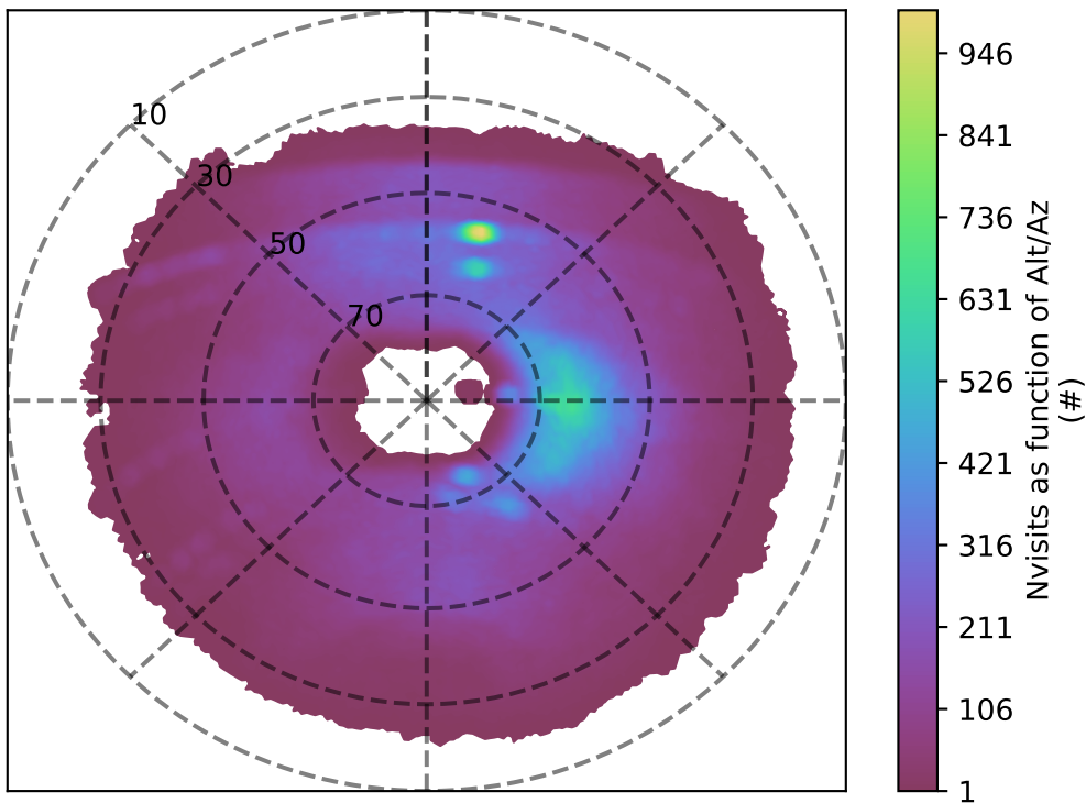
ddf_acor_sf25_lsf40_lsr20_v3.4_10yrs u band: Nvisits as function of Alt/Az
