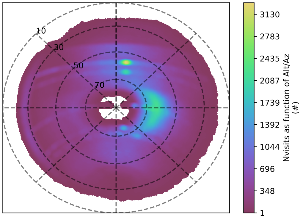
ddf_acor_sf25_lsf40_lsr20_v3.4_10yrs r band: Nvisits as function of Alt/Az
