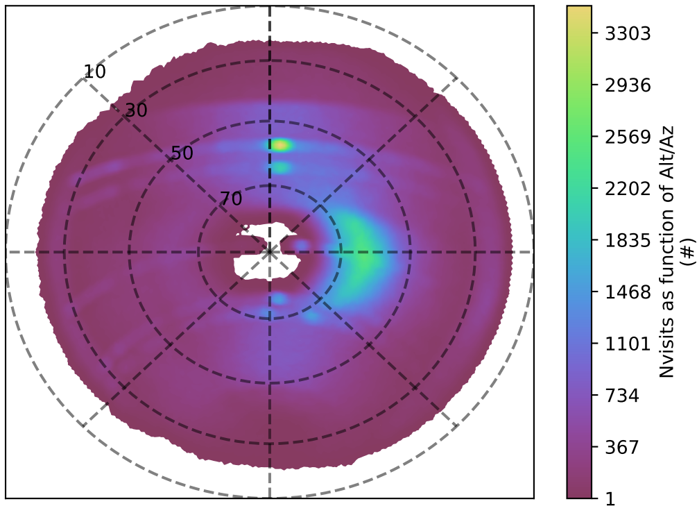
ddf_acor_sf25_lsf40_lsr20_v3.4_10yrs i band: Nvisits as function of Alt/Az
