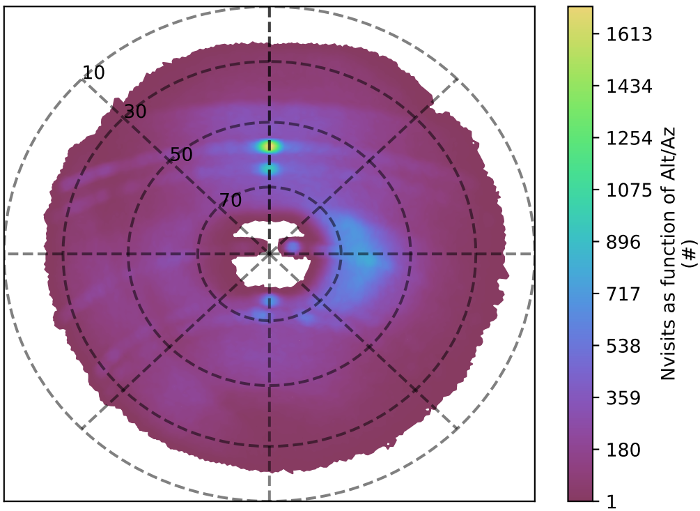
ddf_acor_sf25_lsf40_lsr20_v3.4_10yrs g band: Nvisits as function of Alt/Az
