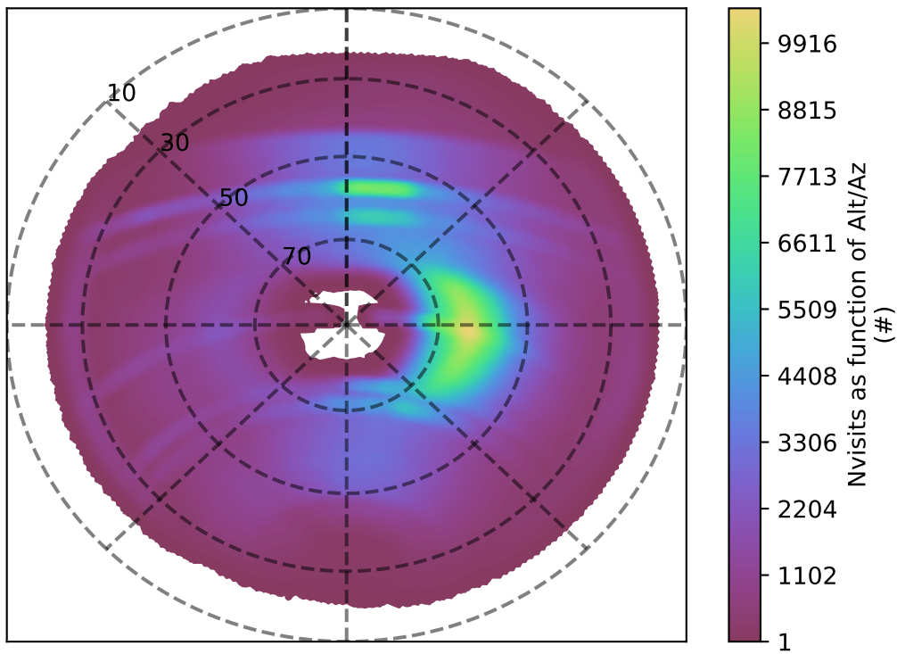
ddf_acor_sf25_lsf40_lsr20_v3.4_10yrs all bands: Nvisits as function of Alt/Az
