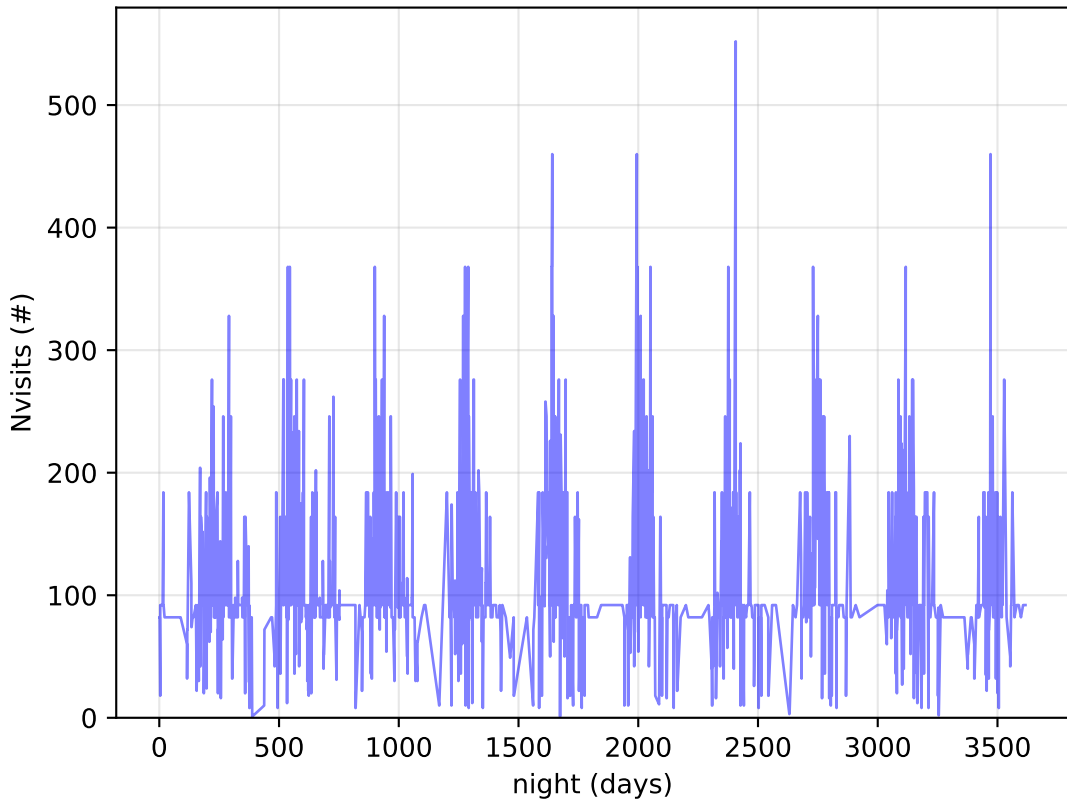
ddf_acor_sf25_ls40_lsr20_v3.4_10yrs DDF: Nvisits
