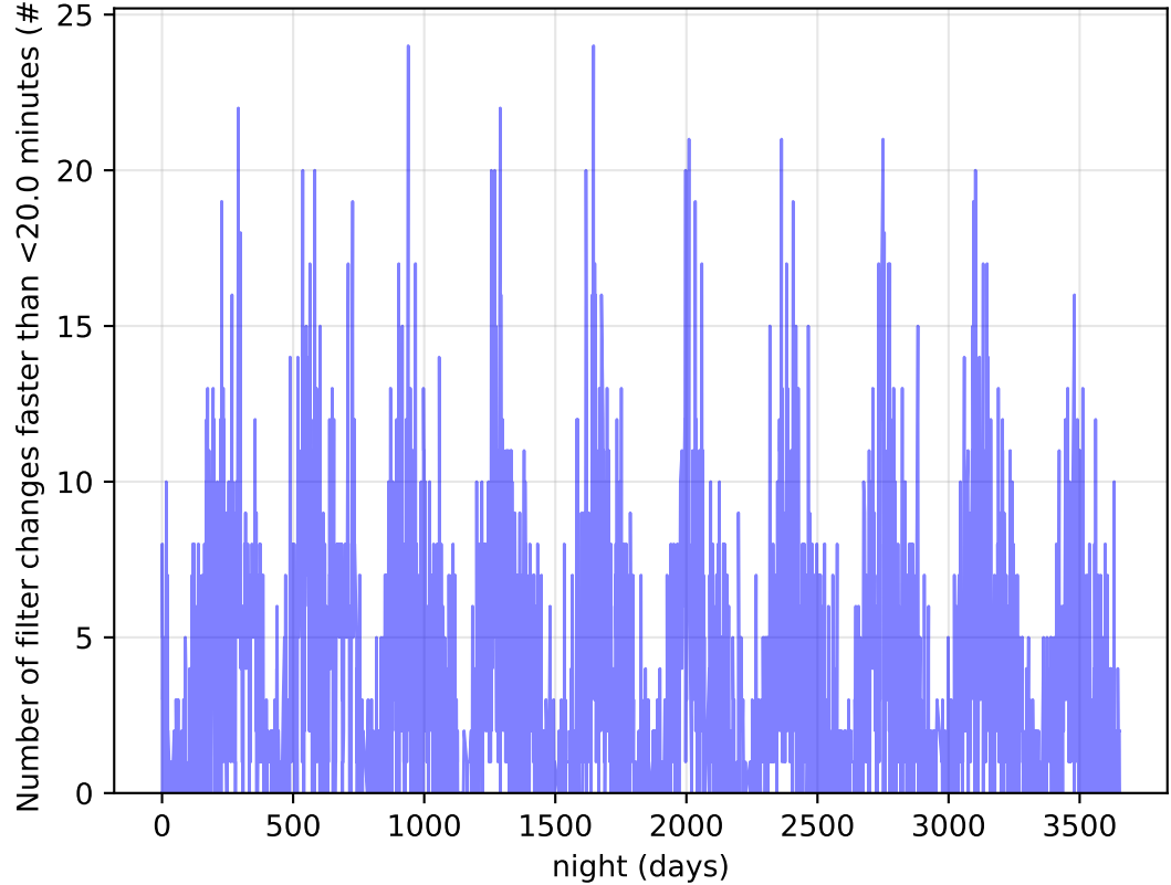
ddf_acor_sf25_Isf40_Isr20_v3.4_10yrs Per Night: Number of filter changes faster than <20.0 minutes
