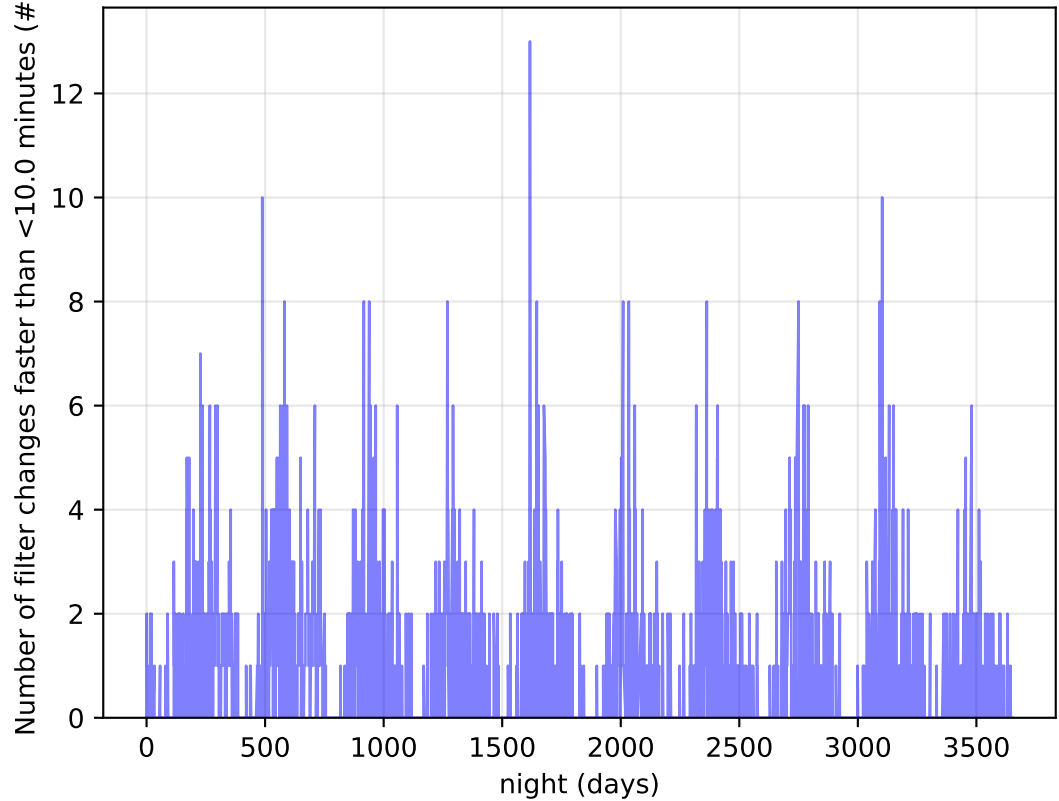
ddf_acor_sf25_Isf40_Isr20_v3.4_10yrs Per Night: Number of filter changes faster than <10.0 minutes
