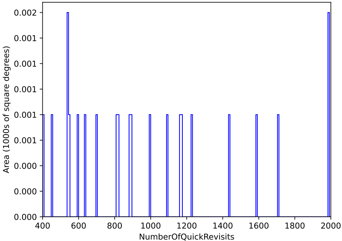
ddf_acor_sf25_lsf40_lsr20_v3.4_10yrs WFD: NumberOfQuickRevisits
