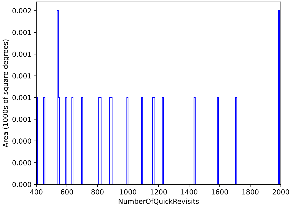
ddf_acor_sf25_Isf40_Isr20_v3.4_10yrs All sky: NumberOfQuickRevisits
