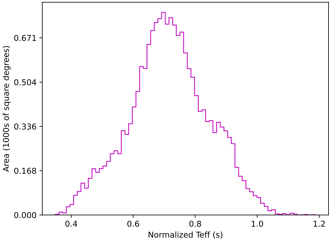
ddf_acor_sf25_lsf40_lsr20_v3.4_10yrs WFD z band: Normalized Teff
