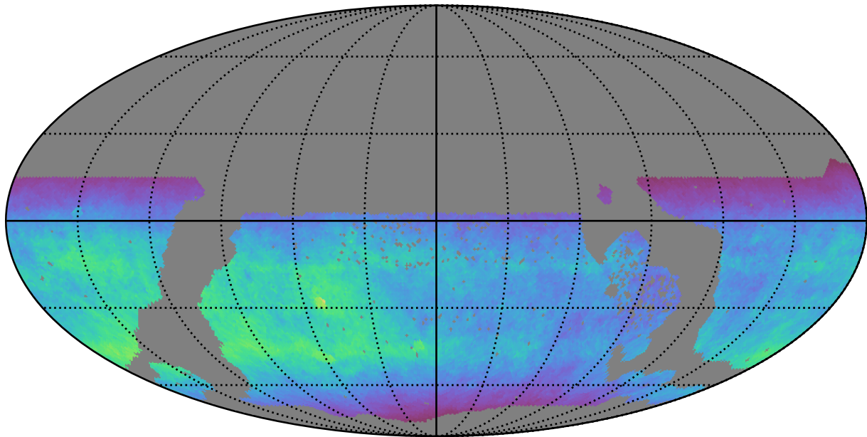
ddf_acor_sf25_lsf40_lsr20_v3.4_10yrs WFD y band: Normalized Teff
