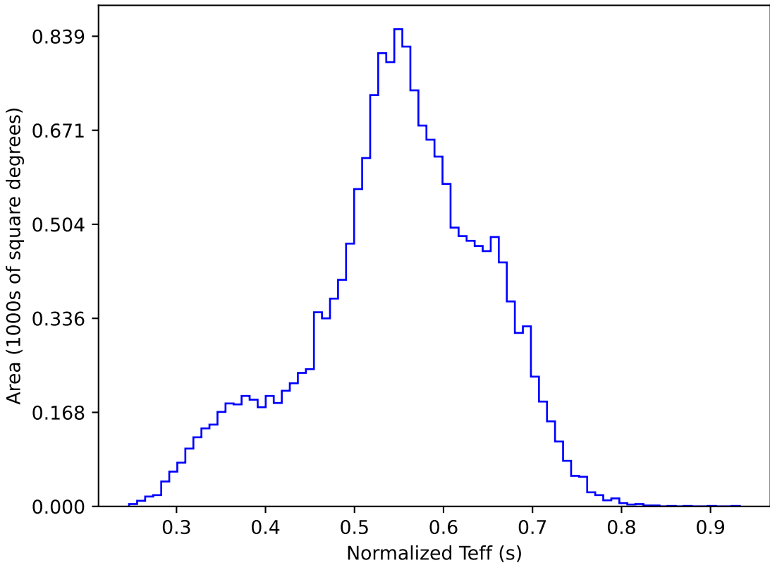
ddf_acor_sf25_lsf40_lsr20_v3.4_10yrs WFD y band: Normalized Teff
