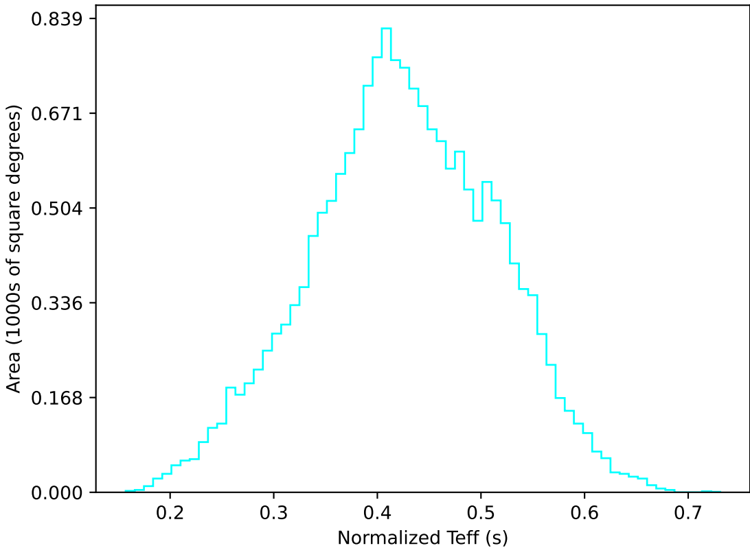
ddf_acor_sf25_ls40_lsr20_v3.4_10yrs WFD u band: Normalized Teff
