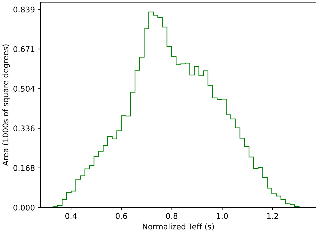
ddf_acor_sf25_lsf40_lsr20_v3.4_10yrs WFD g band: Normalized Teff
