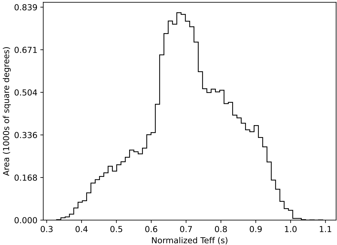
ddf_acor_sf25_lsf40_lsr20_v3.4_10yrs WFD all bands: Normalized Teff
