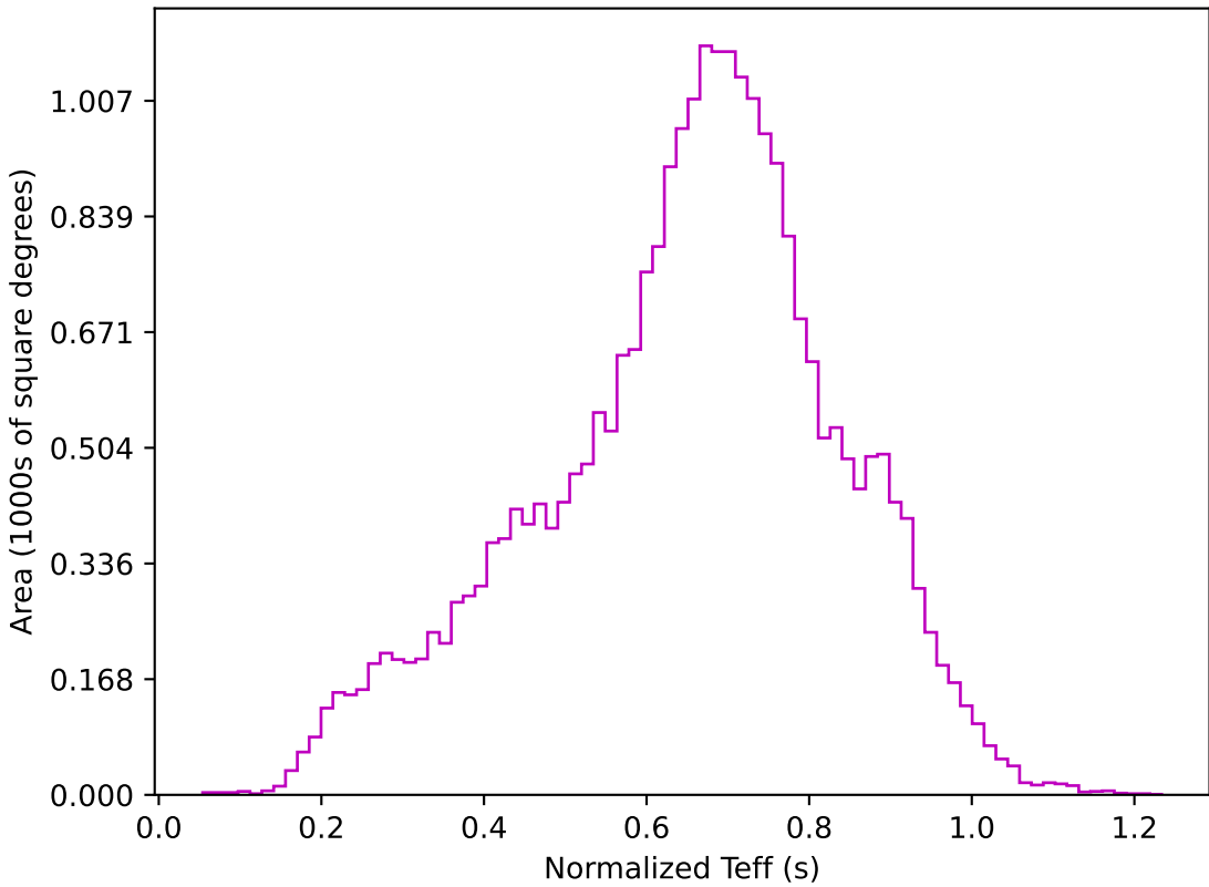
ddf_acor_sf25_lsf40_lsr20_v3.4_10yrs All sky z band: Normalized Teff
