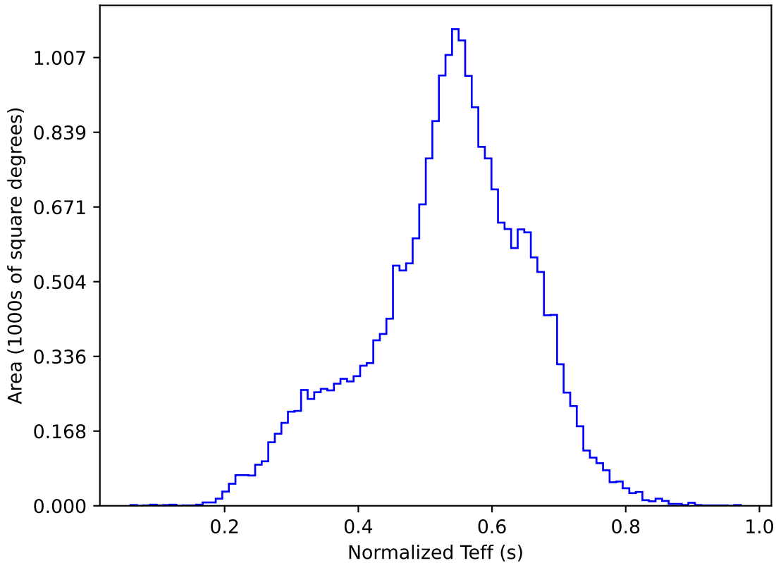
ddf_acor_sf25_lsf40_lsr20_v3.4_10yrs All sky y band: Normalized Teff
