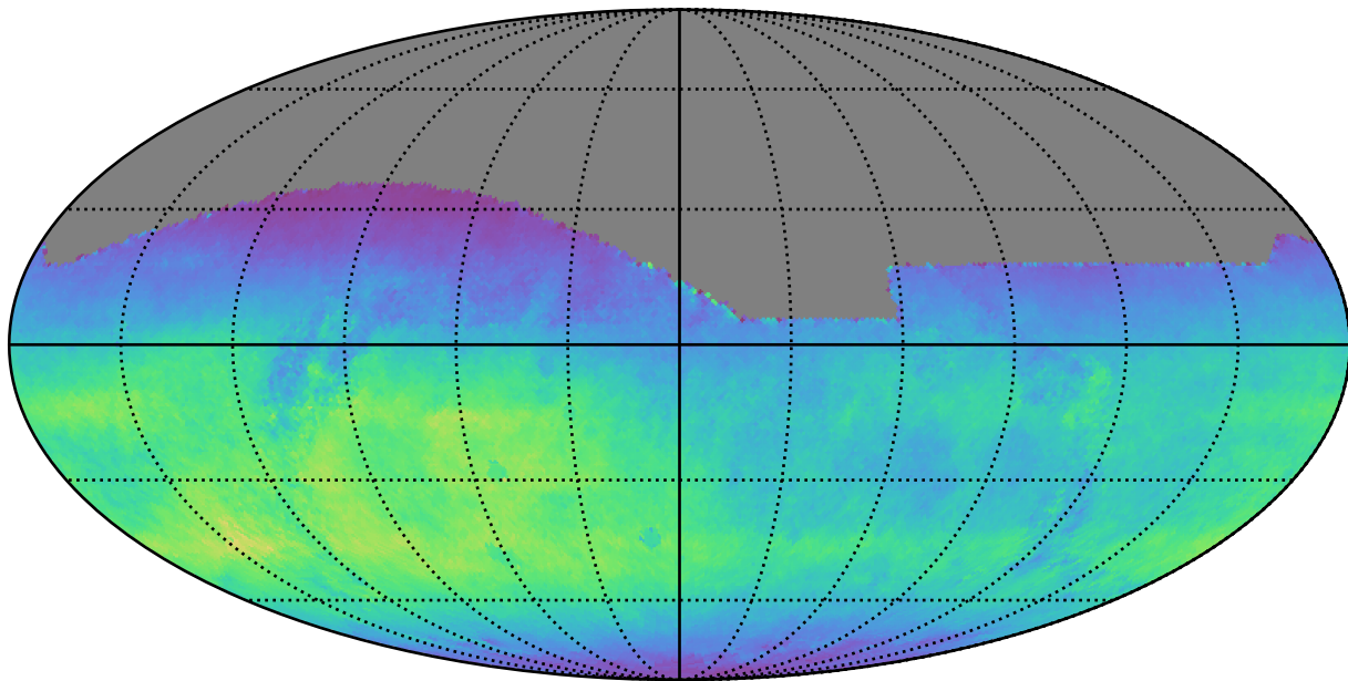
ddf_acor_sf25_lsf40_lsr20_v3.4_10yrs All sky r band: Normalized Teff
