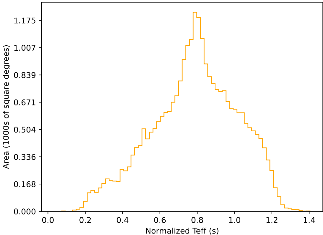
ddf_acor_sf25_lsf40_lsr20_v3.4_10yrs All sky r band: Normalized Teff
