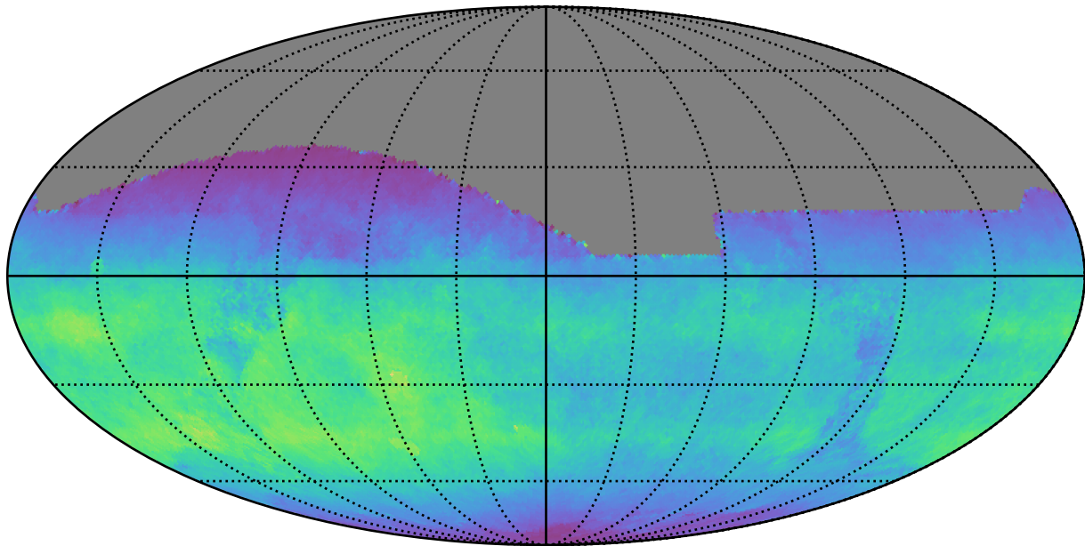
ddf_acor_sf25_lsf40_lsr20_v3.4_10yrs All sky i band: Normalized Teff
