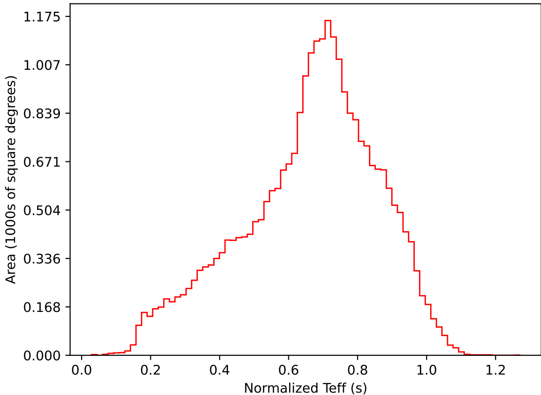
ddf_acor_sf25_lsf40_lsr20_v3.4_10yrs All sky i band: Normalized Teff
